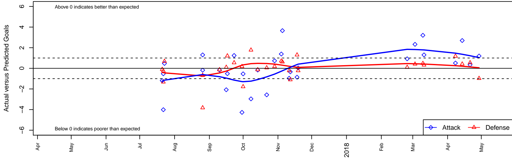
HSC Cosmos B04 Dots are actual minus expected GF (blue circles) and GA (red triangles). Blue line is smoothed change in attack strength. Red is smoothed change in defense strength.
